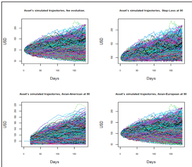
Graph 1 Portfolio's simulated paths with different strategies. Own elaboration with R
